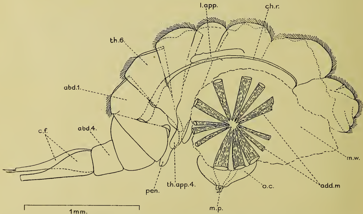
TEXT-FIG. 18.— Baccalaurus digitatus sp. nov. Segmented body from the right-hand side. l.app. , lateral appendage. Other lettering as before.
